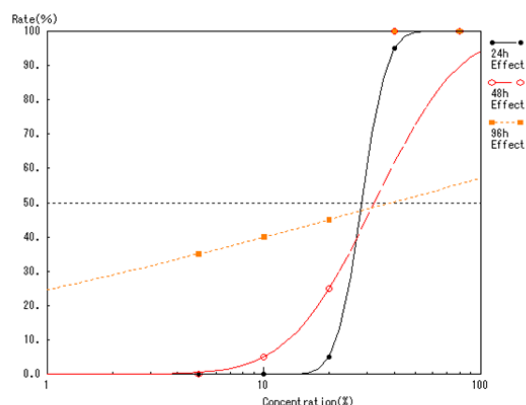
Dose-response curve for EC50 of Daphnia Acute Immobilization Test (Probit method) T処分場_オオミジンコ急性毒性
